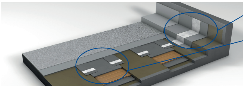
Wecryl 242 Mortar is used to cover the road heating elements and to make good any damage to the surface
