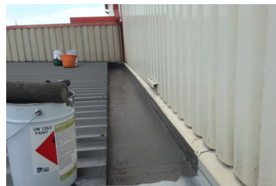
4. Wecryl 230 Thix & Fleece waterproofing installed into the canopy roof gutter
